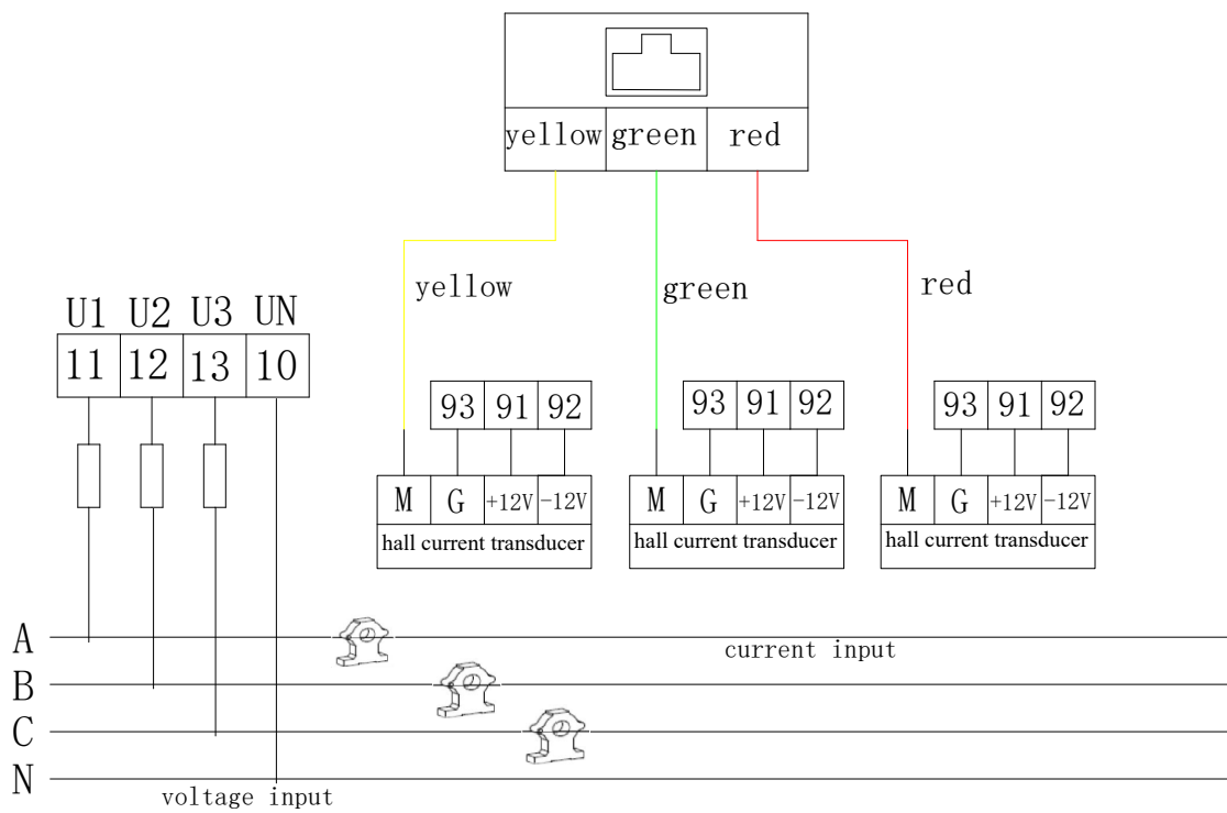
AMB1X0-D(/W)-P1 Discrete Auxiliary Power Supply
